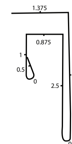
19. F&J CHANNEL
