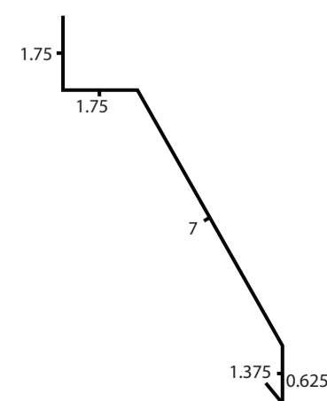
29. TRACK COVER
