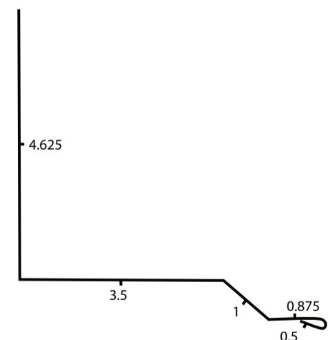
24. SIDEWALL FLASHING
