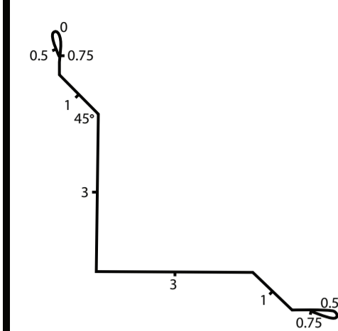
5. 13" I/S CORNER
